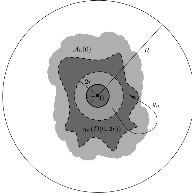
FIGURE 15. Illustration of the proof of the Fatou-Julia Lemma.
