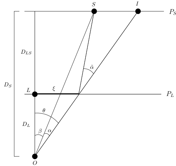
FIGURE 26. S is the light source, I is an image, O is the observer, L is a point mass, P_L is the lens plane, P_S is the source plane.
