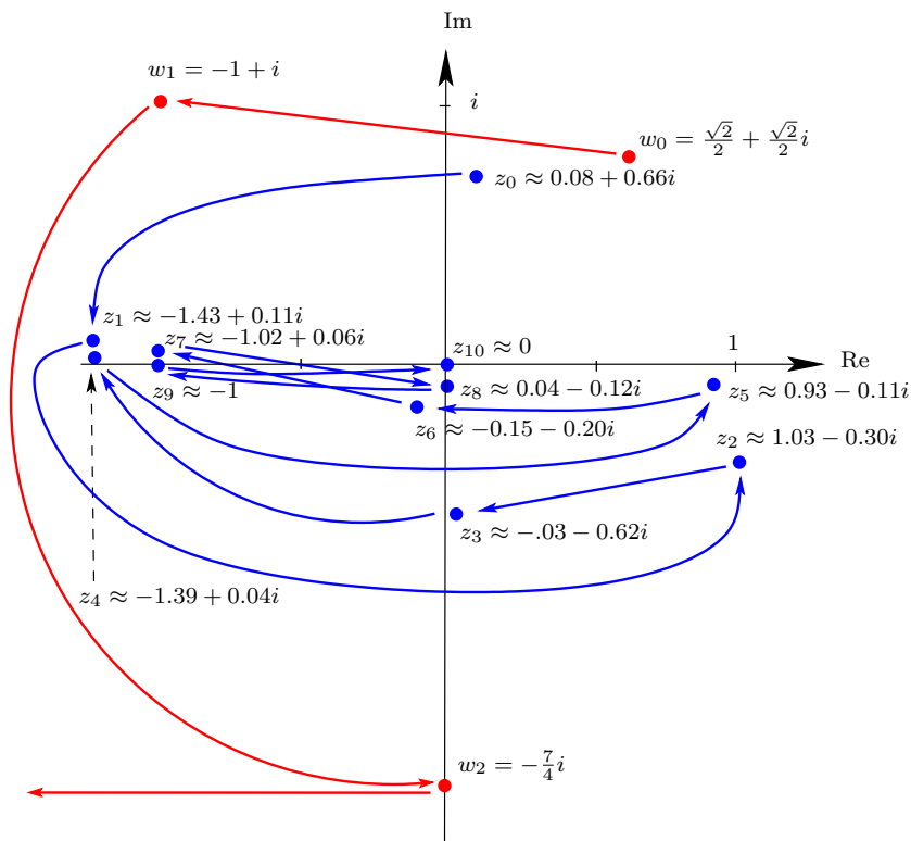
FIGURE 6. Orbits \{z_n\} of z_0 \approx 0.08 + 0.66i and \{w_n\} of w_0 = \frac{\sqrt{2}}{2}(1 + i) under the quadratic polynomial p_{-1}(z) = z^2 - 1 .
