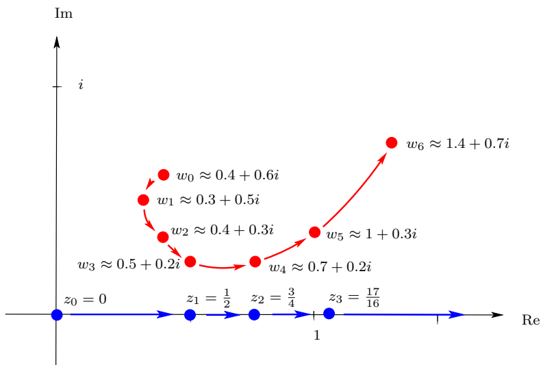
FIGURE 7. Orbits \{z_n\} of z_0 = 0 and \{w_n\} of w_0 \approx 0.4 + 0.6i under the quadratic polynomial p_{\frac{1}{2}}(z) = z^2 + \frac{1}{2} .
