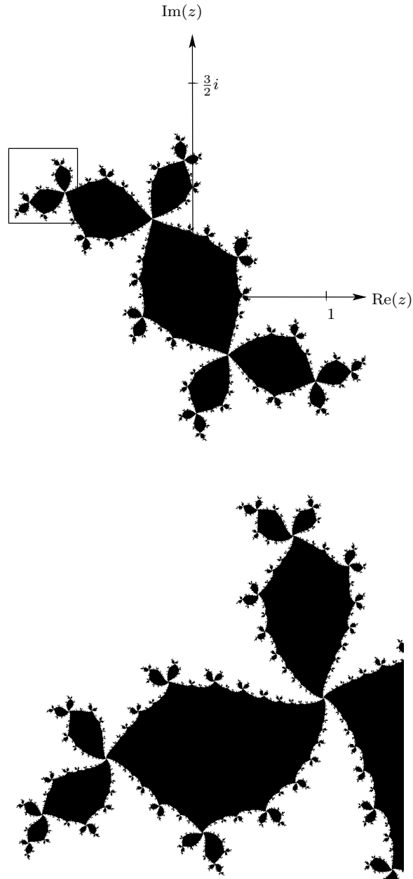
FIGURE 11. Top: basin of attraction of the attracting period 3 cycle 0 \rightarrow c \rightarrow c^2 + c for c \approx -0.12 + 0.75i . Bottom: zoomed-in view of the boxed region from the left.
