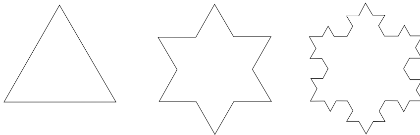
FIGURE 21. The Koch Curve.
