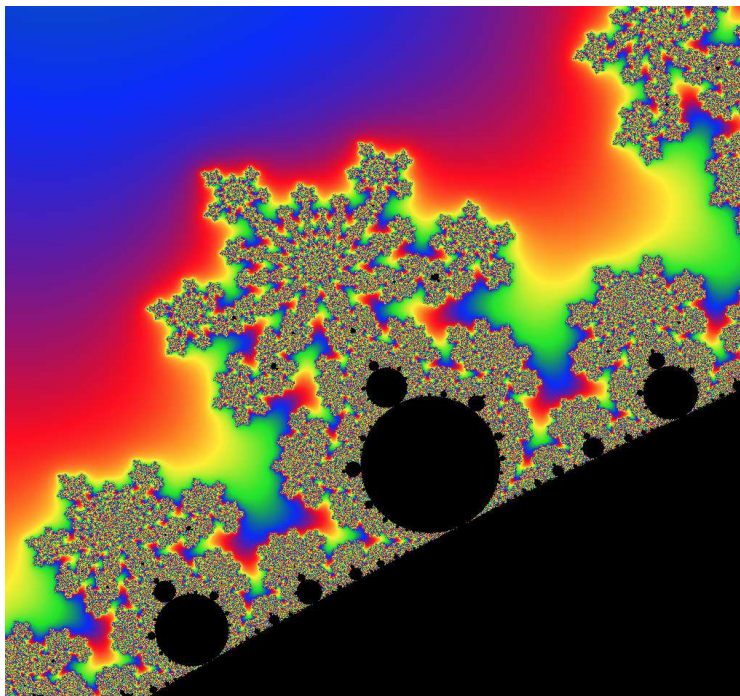
FIGURE 23. Another zoomed-in view of part of the Mandelbrot set.
