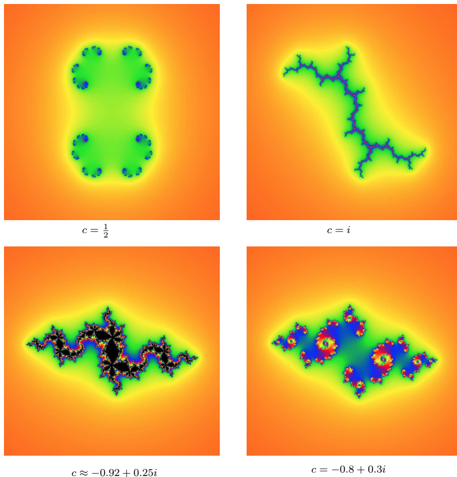
FIGURE 17. Filled Julia sets for four values of c . The basin of attraction for \infty is colored according to the value of G_c(z) .
