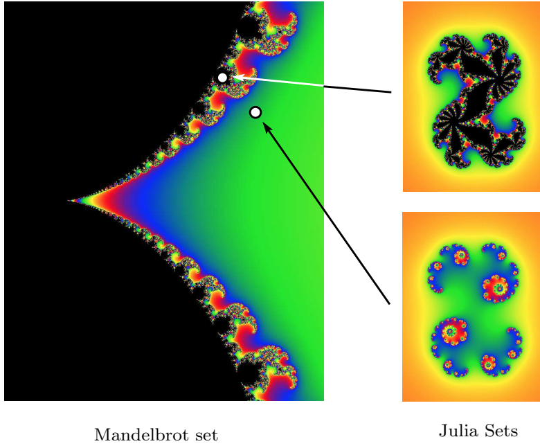
FIGURE 19. Left: Zoomed-in view of the Mandelbrot set near the cusp at c = \frac{1}{4} . Right: two filled Julia sets corresponding to points inside M and outside of M .
