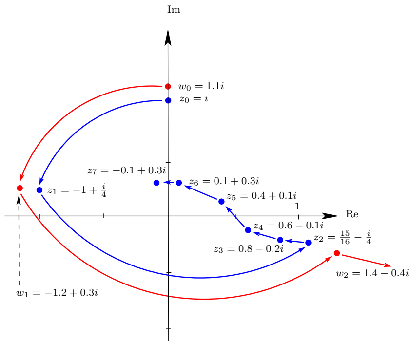
FIGURE 5. Orbits \{z_n\} for initial condition z_0 = i and \{w_n\} for w_0 = 1.1i under p(z) = z^2 + \frac{i}{4} .
