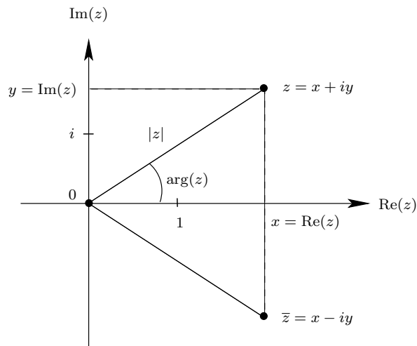
FIGURE 1. The complex plane.
