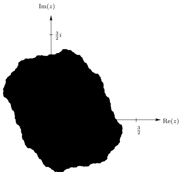
FIGURE 9. Basin of attraction of the fixed point z_* = \frac{1}{2} - \frac{\sqrt{1-i}}{2} for p(z) = z^2 + \frac{i}{4} .
