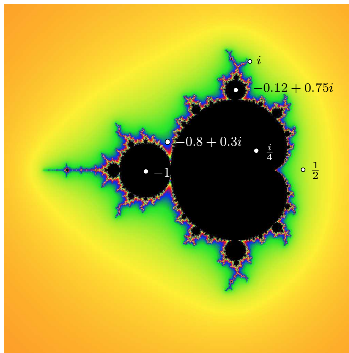
FIGURE 18. Mandelbrot set with the approximate locations of parameters c = \frac{i}{4}, -1, -0.12 + 0.75i, i, -0.8 + 0.3i, and \frac{1}{2} labeled.
