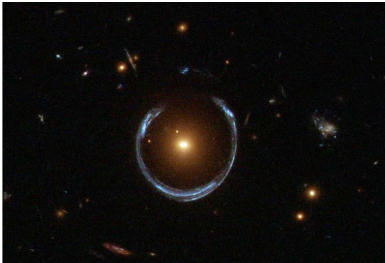
FIGURE 24. An Einstein Ring. For more information, see http://apod.nasa.gov/apod/ap111221.html .
