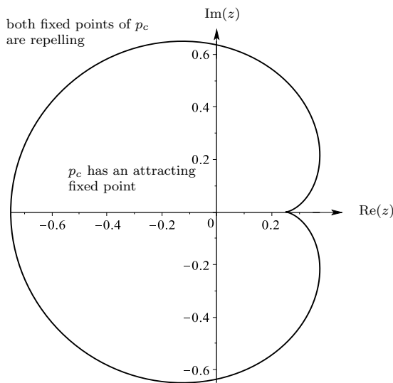
FIGURE 13. p_c(z) = z^2 + c has an attracting fixed point if and only if c lies inside the Cardioid c = \frac{e^{i\theta}}{2} - \frac{e^{i2\theta}}{4} , where 0 \leq \theta \leq 2\pi , depicted here.
