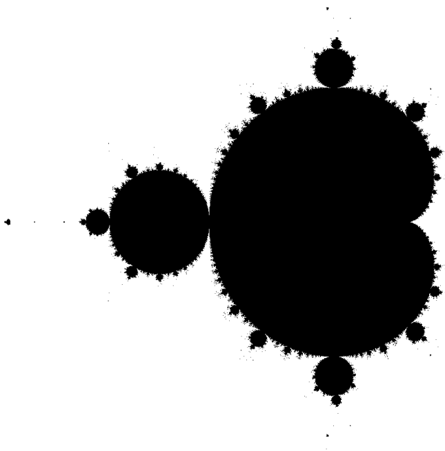
FIGURE 16. The Mandelbrot set M , shown in black. The region shown is approximately -2.4 \leq \operatorname{Re}(z) \leq 1 and -1.6 \leq \operatorname{Im}(z) \leq 1.6 .
