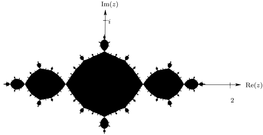
FIGURE 10. Basin of attraction of the period two cycle 0 \leftrightarrow -1 for p(z) = z^2 - 1 .
