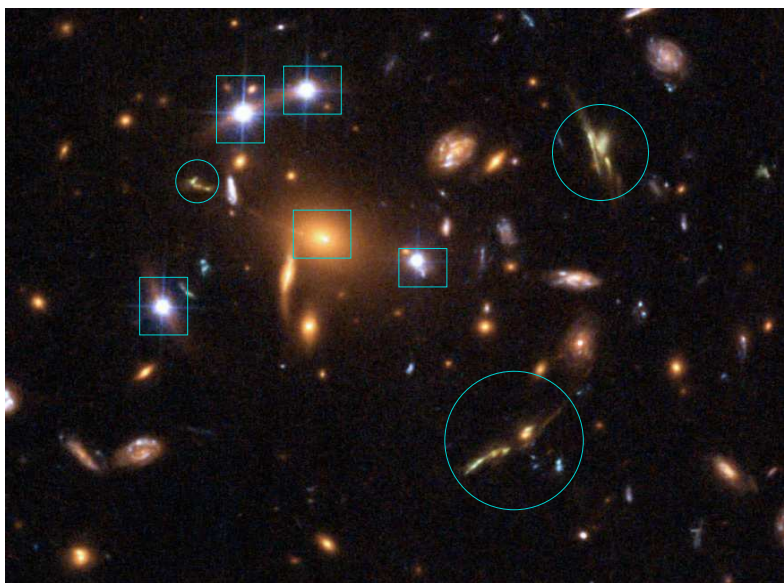
FIGURE 25. Five images of the same quasar (boxed) and three images of the same galaxy (circled). The middle image of the quasar (boxed) is behind the small galaxy that does the lensing. For more information, see http://www.nasa.gov/multimedia/imagegallery/image_feature_575.html
