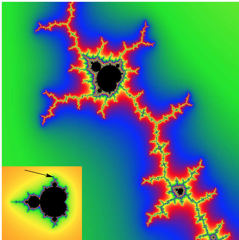
FIGURE 22. Zoomed-in view of part of the Mandelbrot set showing two smaller copies. The approximate location where we have zoomed in is marked by the tip of the arrow in the inset figure.
