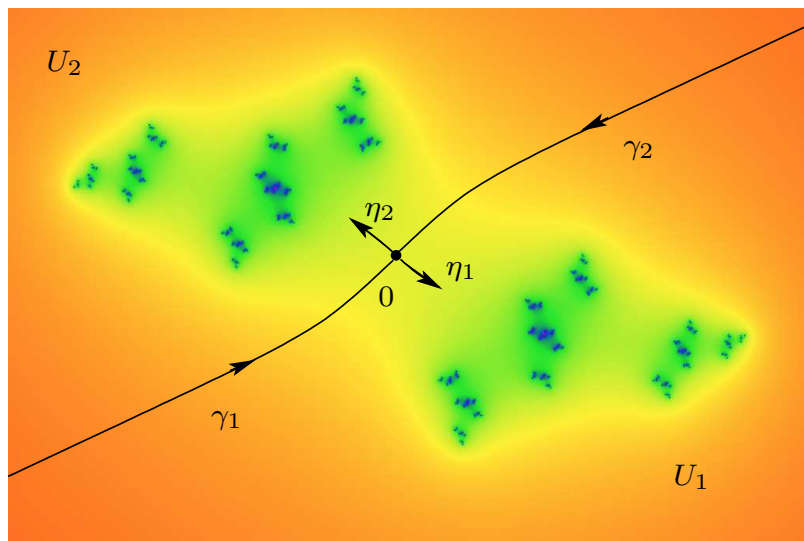
FIGURE 20. Stable and unstable trajectories of -\nabla G_c for the critical point 0.
