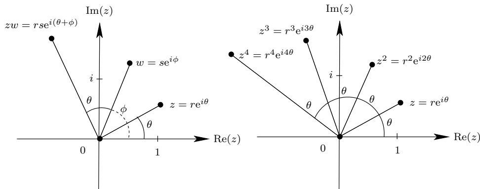
FIGURE 2. Multiplication and taking powers in polar form.
