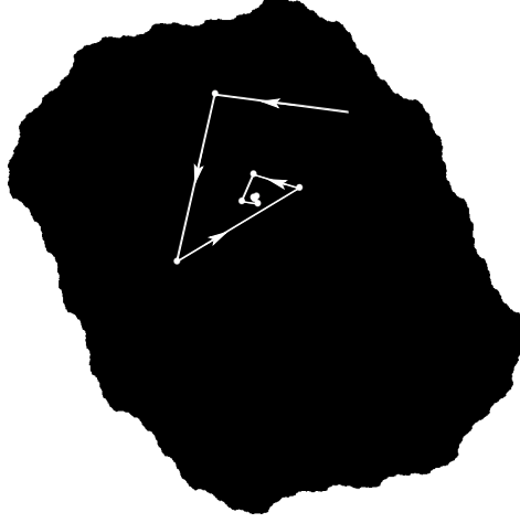
FIGURE 12. An orbit converging to the attracting fixed point for p(z) = z^2 + \frac{i}{4} . Here, \lambda = 1 - \sqrt{1 - 2i} \approx 0.8e^{1.9i} .
