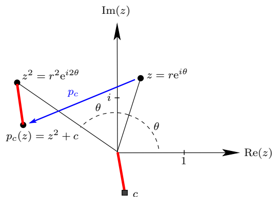
FIGURE 4. Geometric interpretation of applying p_c(z) = z^2 + c .
