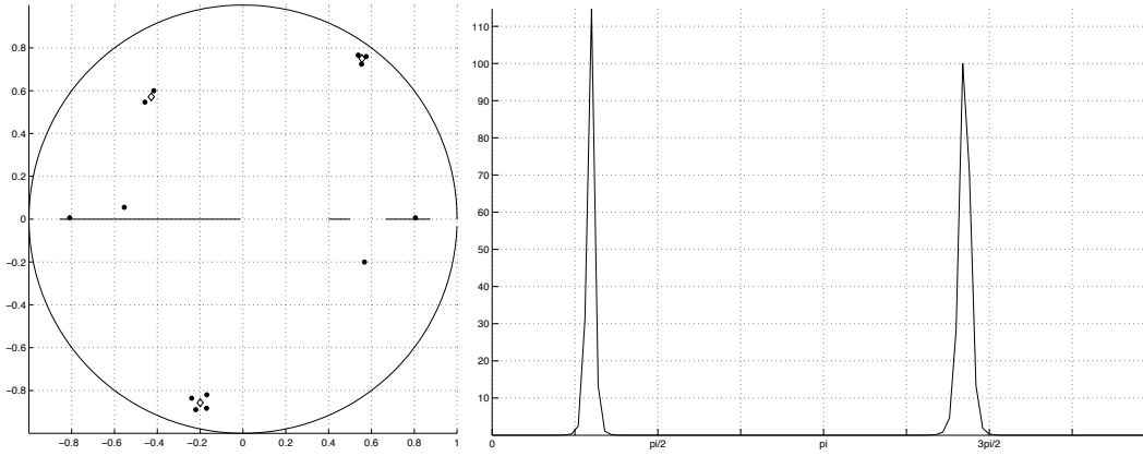
FIGURE 1. Poles of \Pi_{13} and the error |F - \Pi_{13}| on \mathbb{T}
