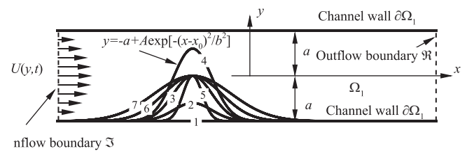
Fig. 1. Schematic representation of a 2D stenosed artery. The geometrical parameters are: (1) A/a=0 (channel flow), (2) A/a=0.4 and b/a=1.0 , (3) A/a=1.0 and b/a=1.0 , (4) A/a=1.6 and b/a=1.0 , (5) A/a=1.0 and b/a=0.5 , (6) A/a=1.0 and b/a=1.5 , and (7) A/a=1.0 and b/a=2.0 .
