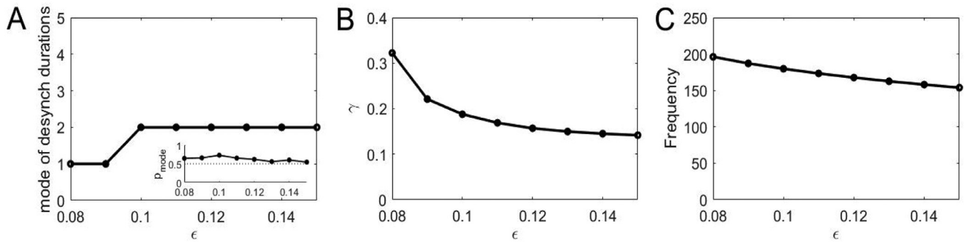
Fig. 1. The effect of \epsilon (the ratio of the predation rate to the intrinsic prey growth rate). (A) Mode value of the durations of desynchronization events (the main graph) and the corresponding probability to observe the mode value p_{mode} (the insert). The high (close to one) value of probability to observe a mode indicates that the desynchronizations of corresponding duration are strongly prevalent. (B) Synchronization strength index \gamma . (C) The mean frequency of oscillations in coupled predator-prey oscillators. The other parameters are \alpha = 0.34 , \eta = 0.32 , d = 0.03 , ratio \sigma = 0.19 .
